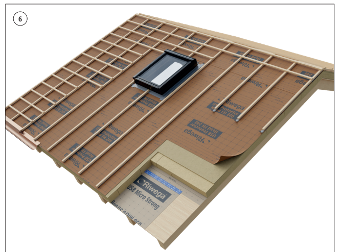
Finally, proceed with the placement of the remaining counter-battens and roof tile holder slats
